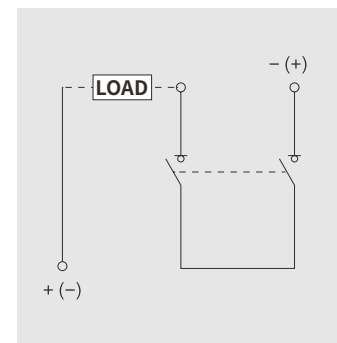
Wiring method 4
