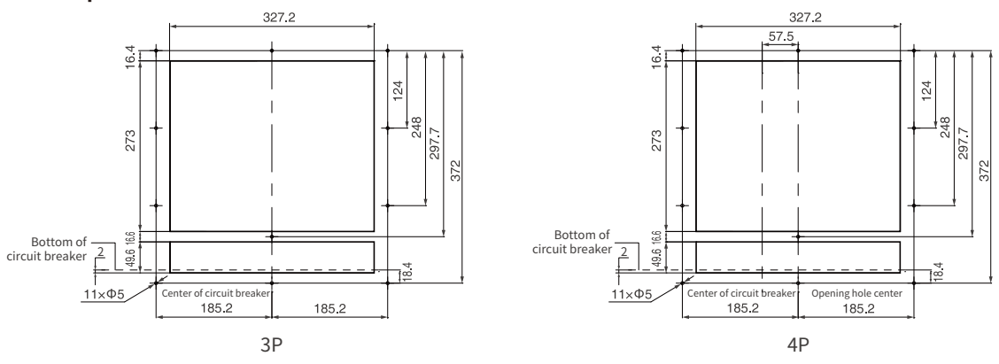
Cabinet door open hole dimension
