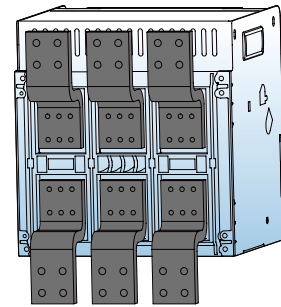
Forward Wiring C3
