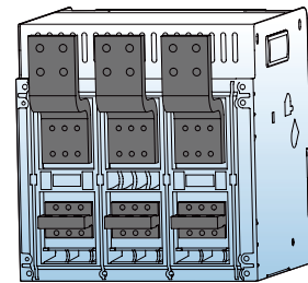
Mixed Wiring C6 (Upper Forward, Lower Horizontal)
